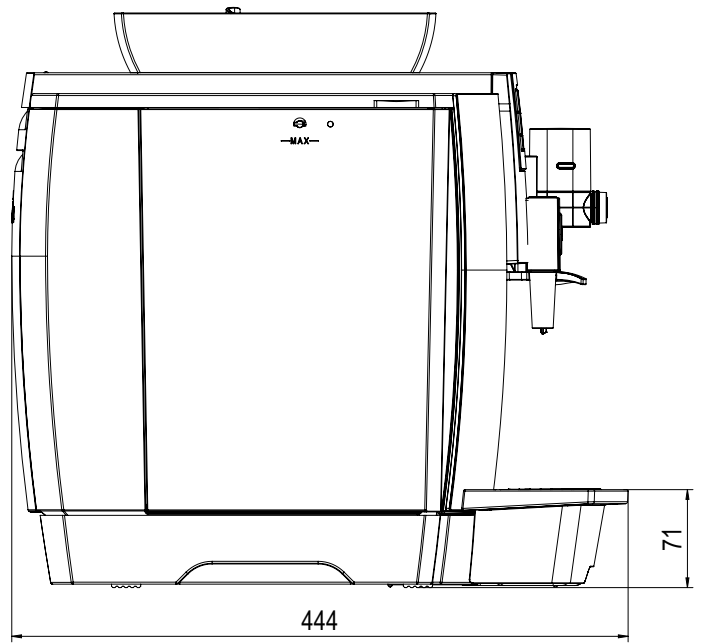
Side outline
